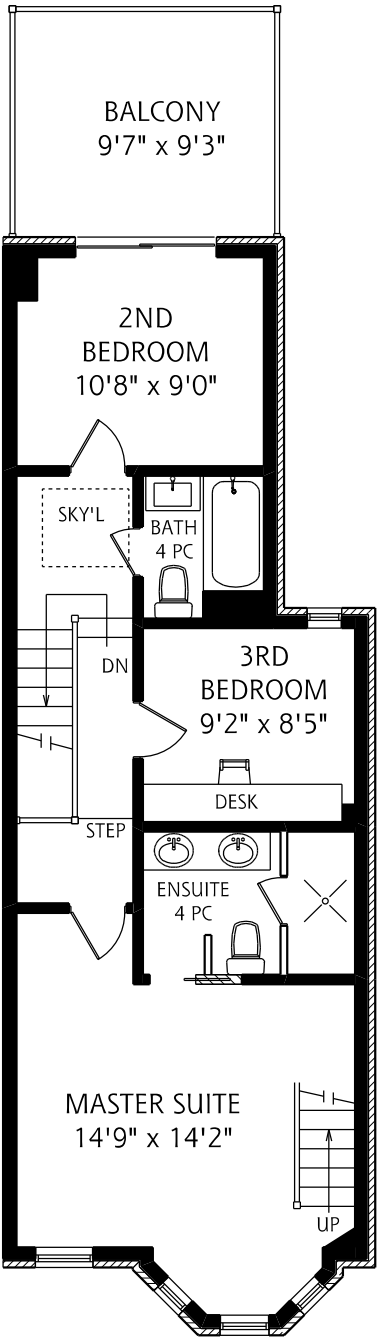
SECOND FLOOR 680 SQUARE FEET
